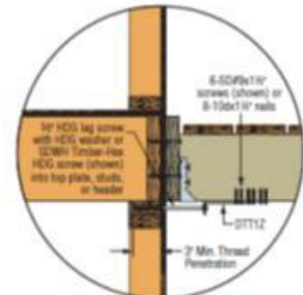
Typical DTT1Z Deck-to-House Lateral Load Connection For more information on lateral load connections, see technical bulletin T-DECKLALOAD
